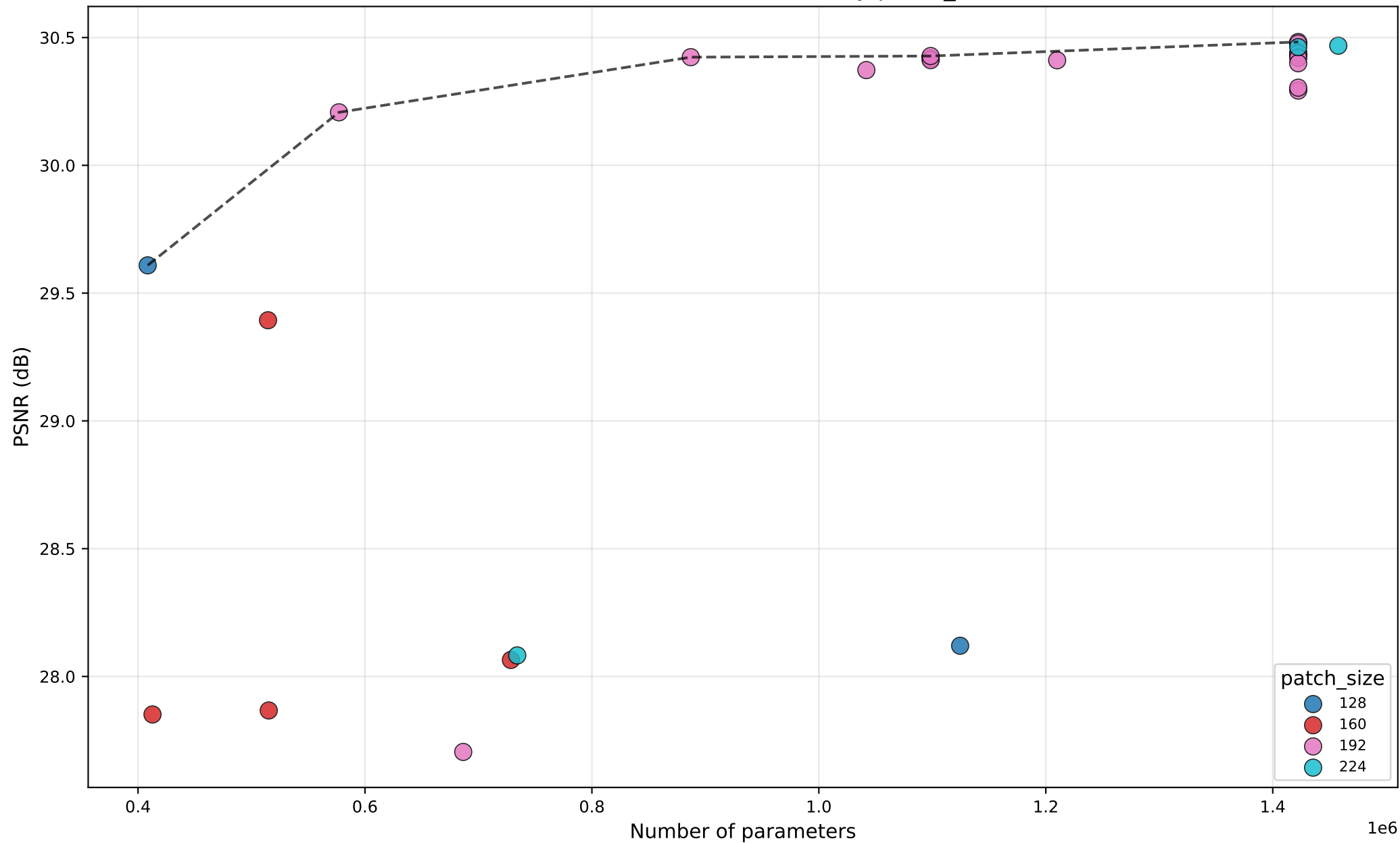
PSNR vs #Params — SwinT — by patch_size
